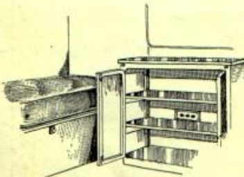
Ventilated food locker, shown above, is placed between the two single beds in the rear of the caravan. The front of this cabinet serves as a mounting for the table.
